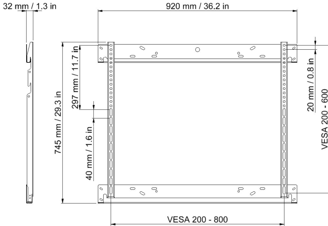
Configuration when mounted on BalanceBox 400 and Mobile Stand Mix
